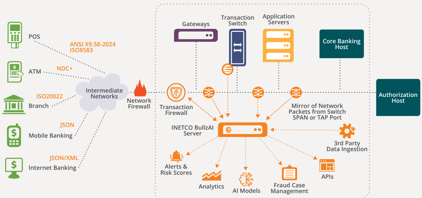
DIAGRAM: INETCO BullzAI captures, decodes and correlates in-flight transactions to detect and prevent payment fraud, money laundering and cyber-attacks in real-time. Spot unusual transaction patterns, path deviations, message manipulation and compromised systems before the damage is done.
